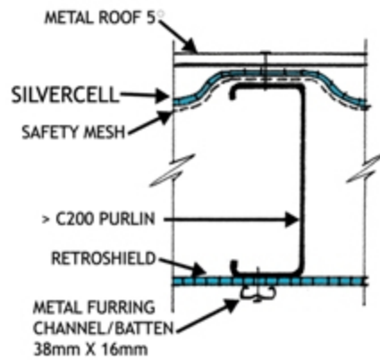
METAL ROOF 5° PITCH
