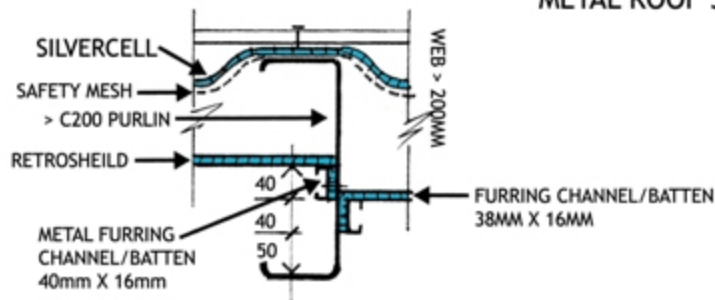
METAL ROOF 5° PITCH
